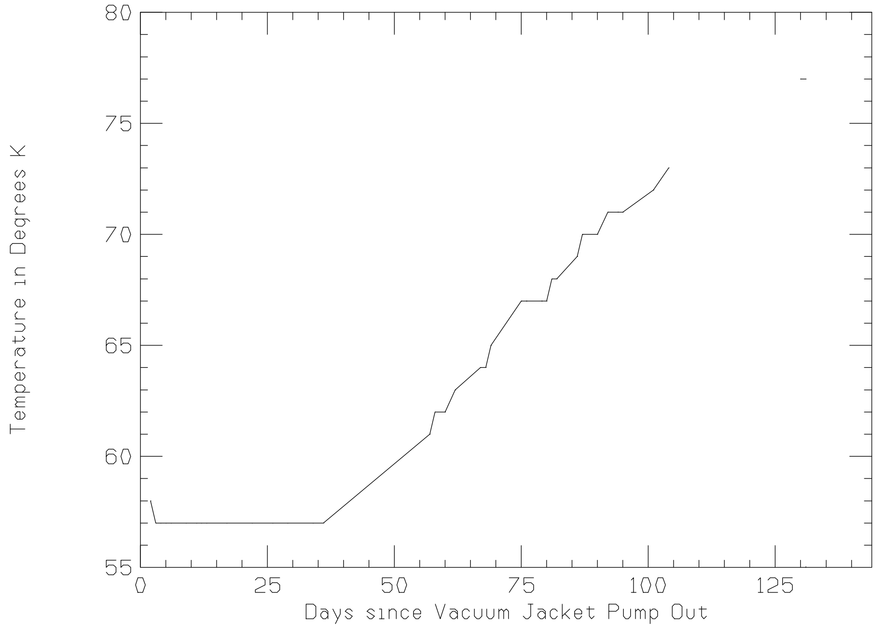
Purifier Cold Trap Temperature Since Vacuum Jacket Pump Out on 26-Aug-2022
