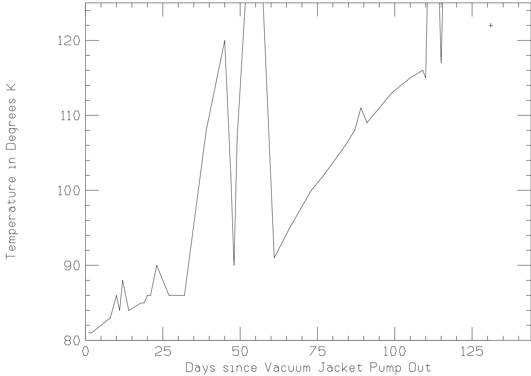
Purifier Heat Exchanger Temperature Since Vacuum Jacket Pump Out on 7-Apr-2023
