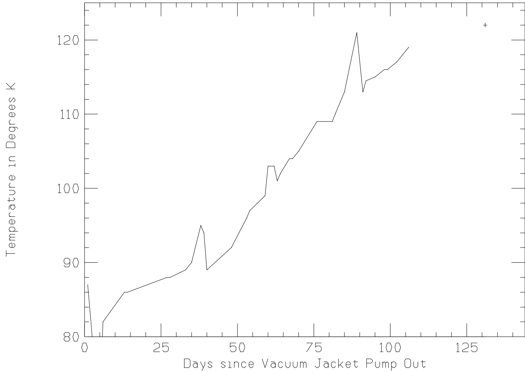
Purifier Heat Exchanger Temperature Since Vacuum Jacket Pump Out on 15-Dec-2022
