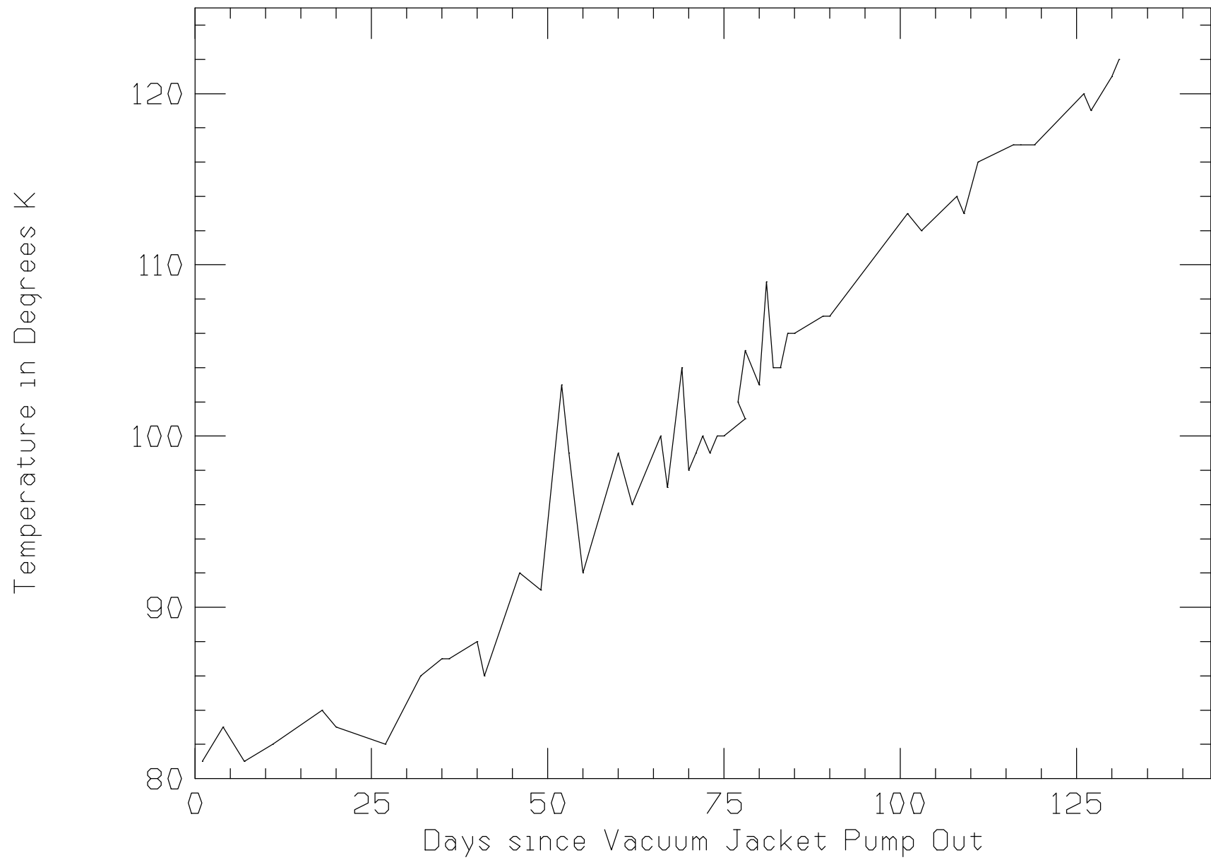
Purifier Heat Exchanger Temperature Since Vacuum Jacket Pump Out on 15-April-2022
