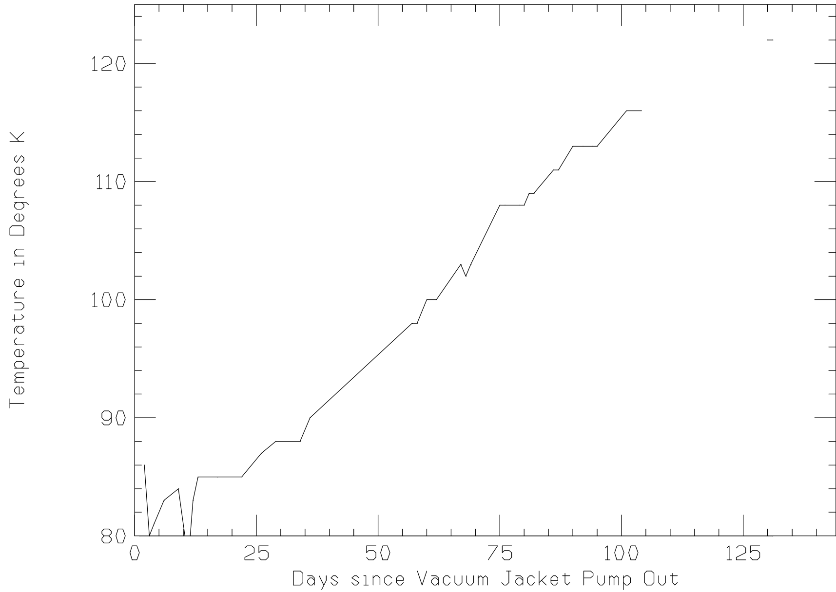
Purifier Heat Exchanger Temperature Since Vacuum Jacket Pump Out on 26-Aug-2022
