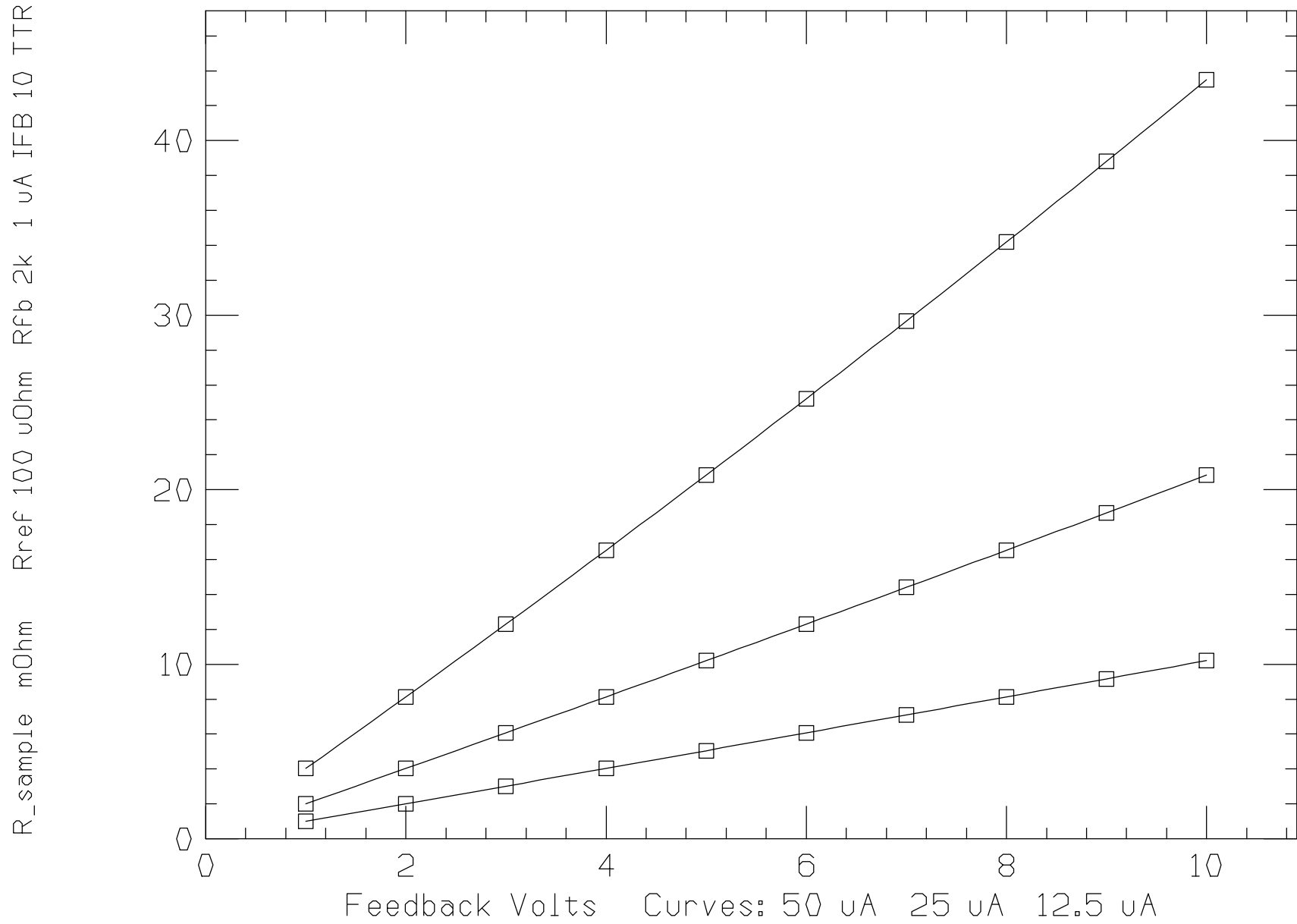
R_sample vs Feedback Voltage at Various Sweeper Currents 9-Nov-2020
