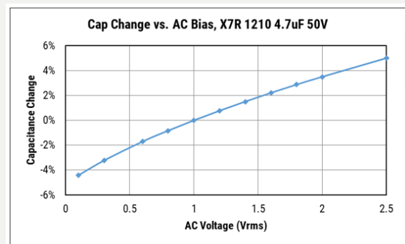
Figure 5 – Capacitance Change vs. AC Bias X7R 1210 4.7uF 50V
