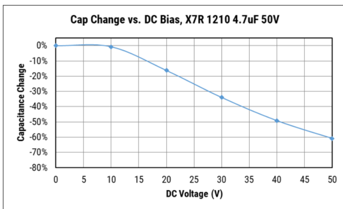
Figure 1 – Capacitance Change vs. DC Bias X7R 1210 4.7uF 50V
