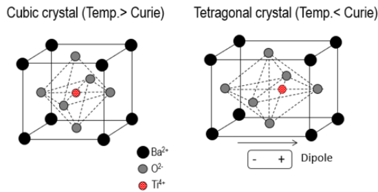
Figure 3 - BaTiO 3 above and below Curie Point
