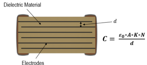
Figure 2 - Cross Section of MLCC
