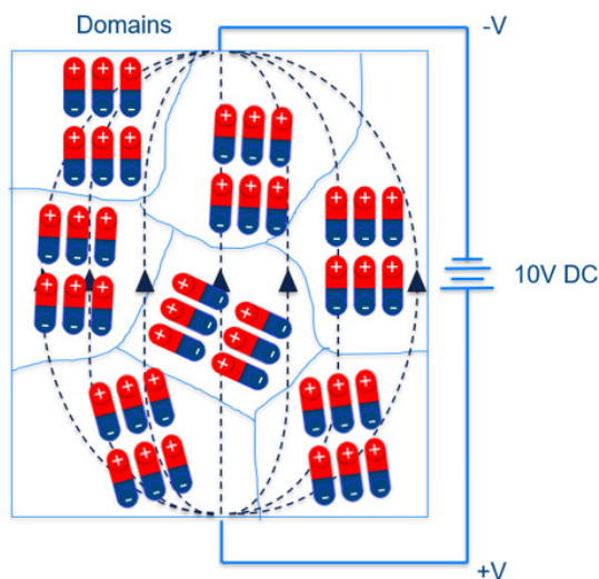
Figure 4 – BaTiO 3 under the influence of an electric field
