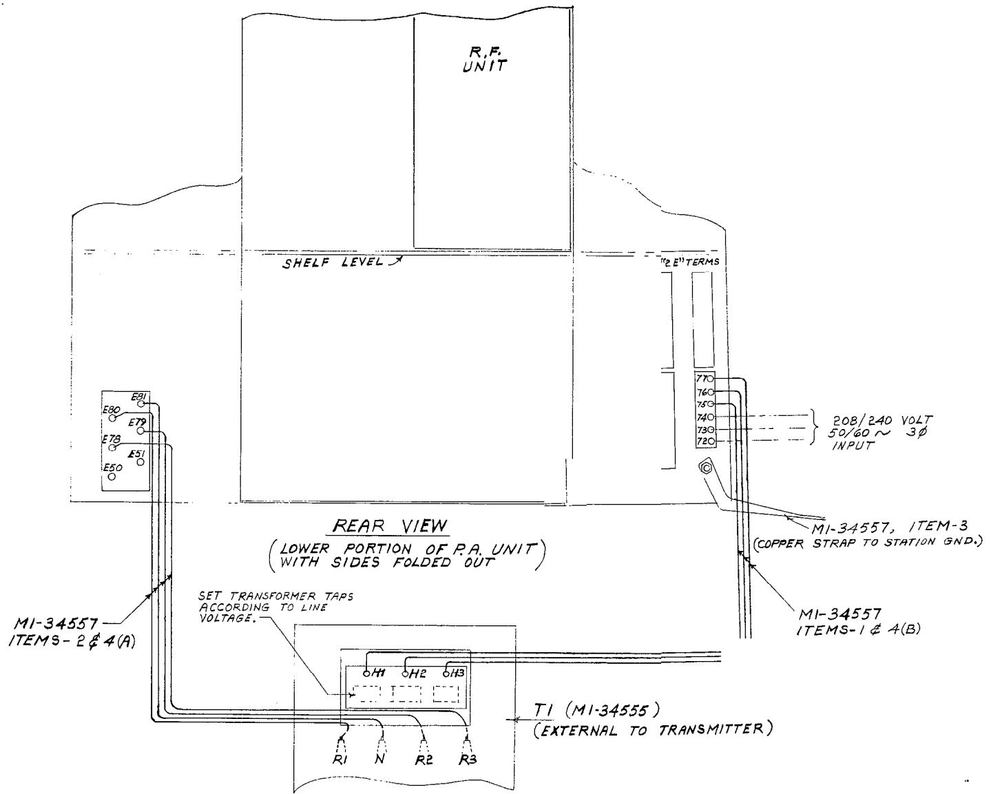
Figure T-26. Installation/Wiring. Plate Transformer (8729601)
