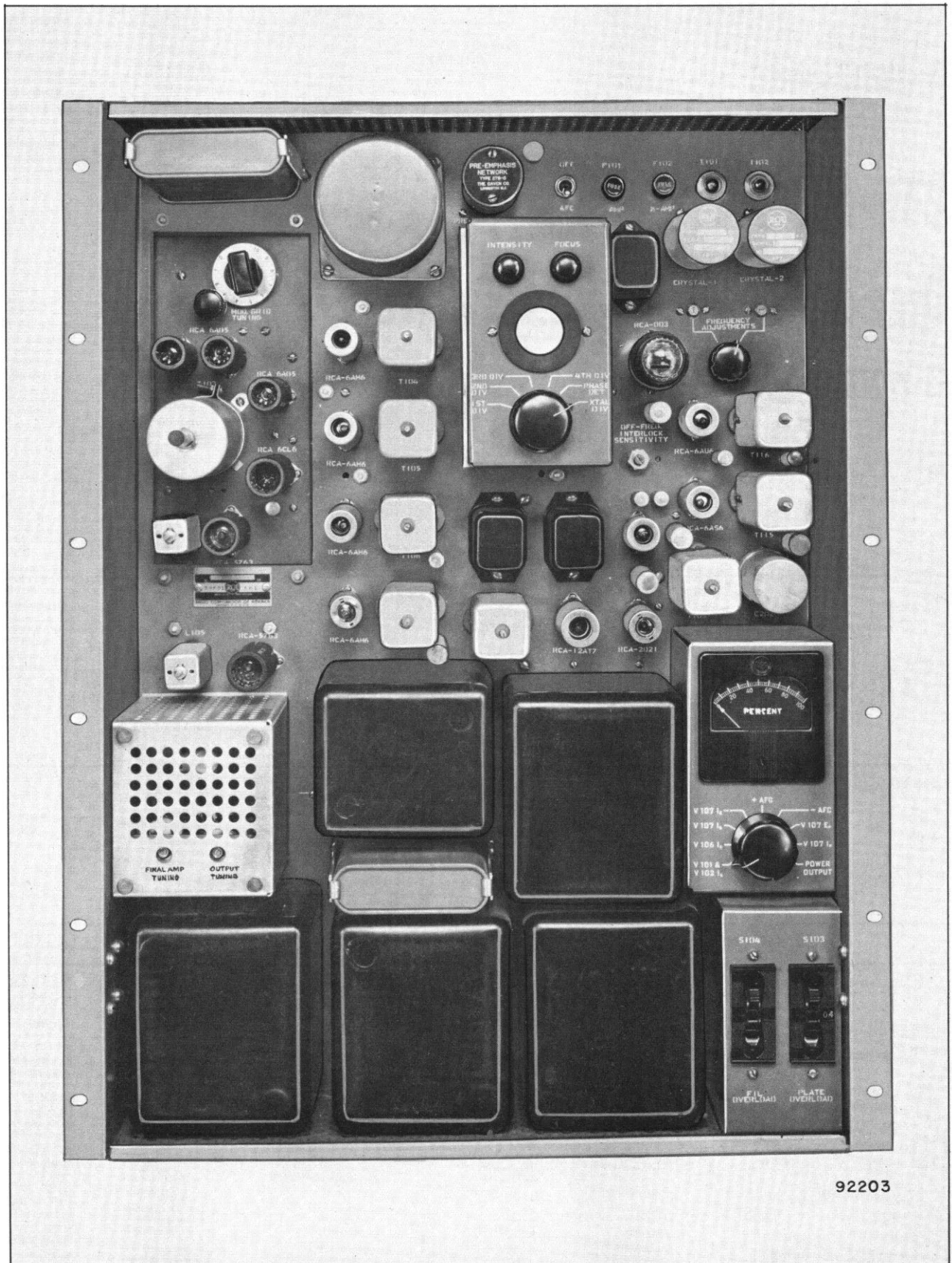
Figure E-1. BTE-10B FM Multiplex Exciter
