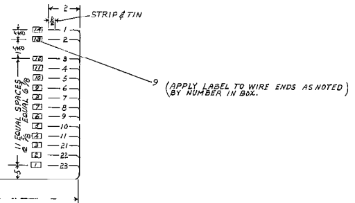
Figure T-23. Cable Assembly and Connections (18616018)
