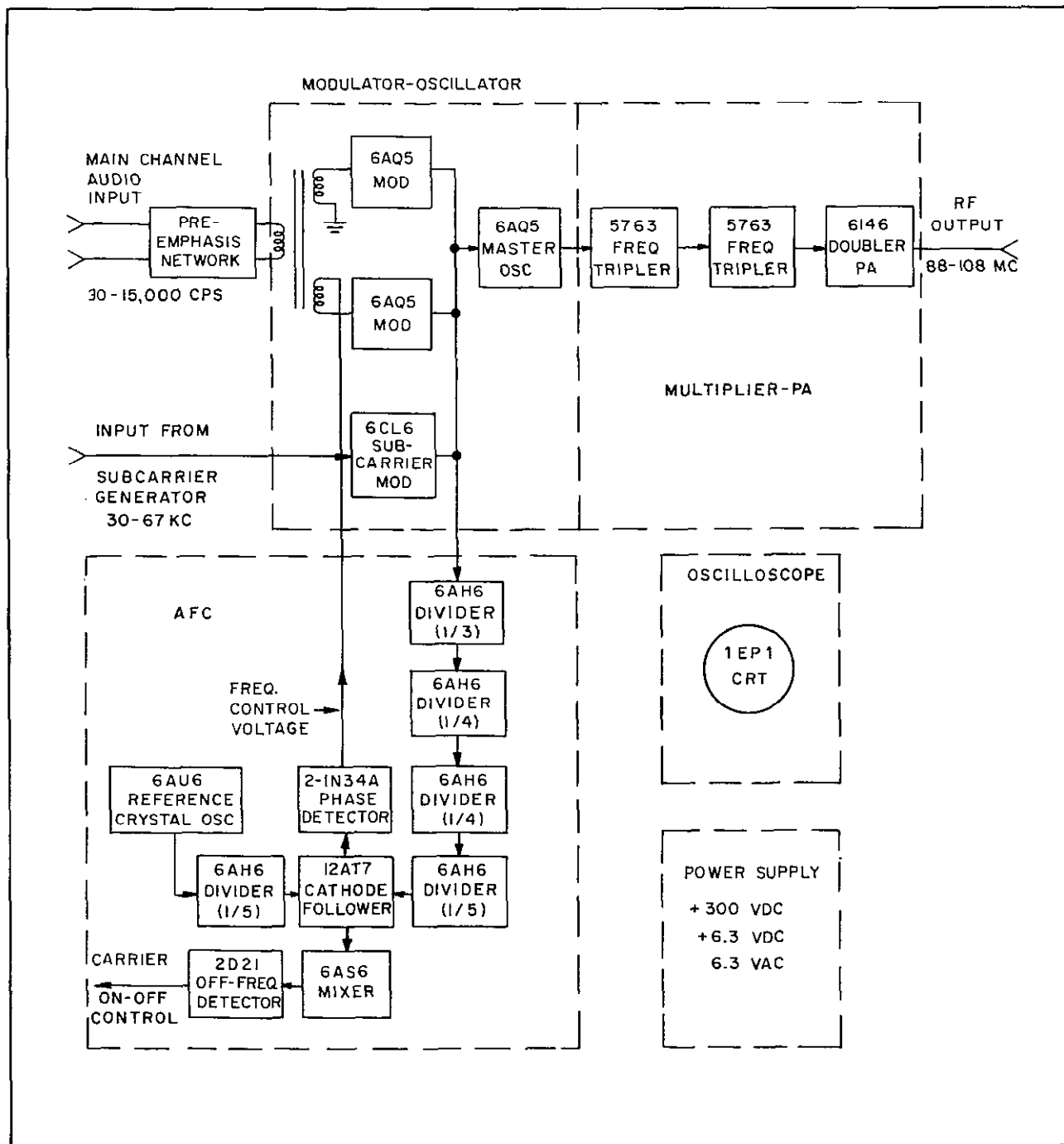
Figure E-2. Block Diagram, BTE-10B FM Exciter
