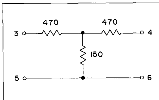
Figure E-8. Schematic, 18 db Attenuator
