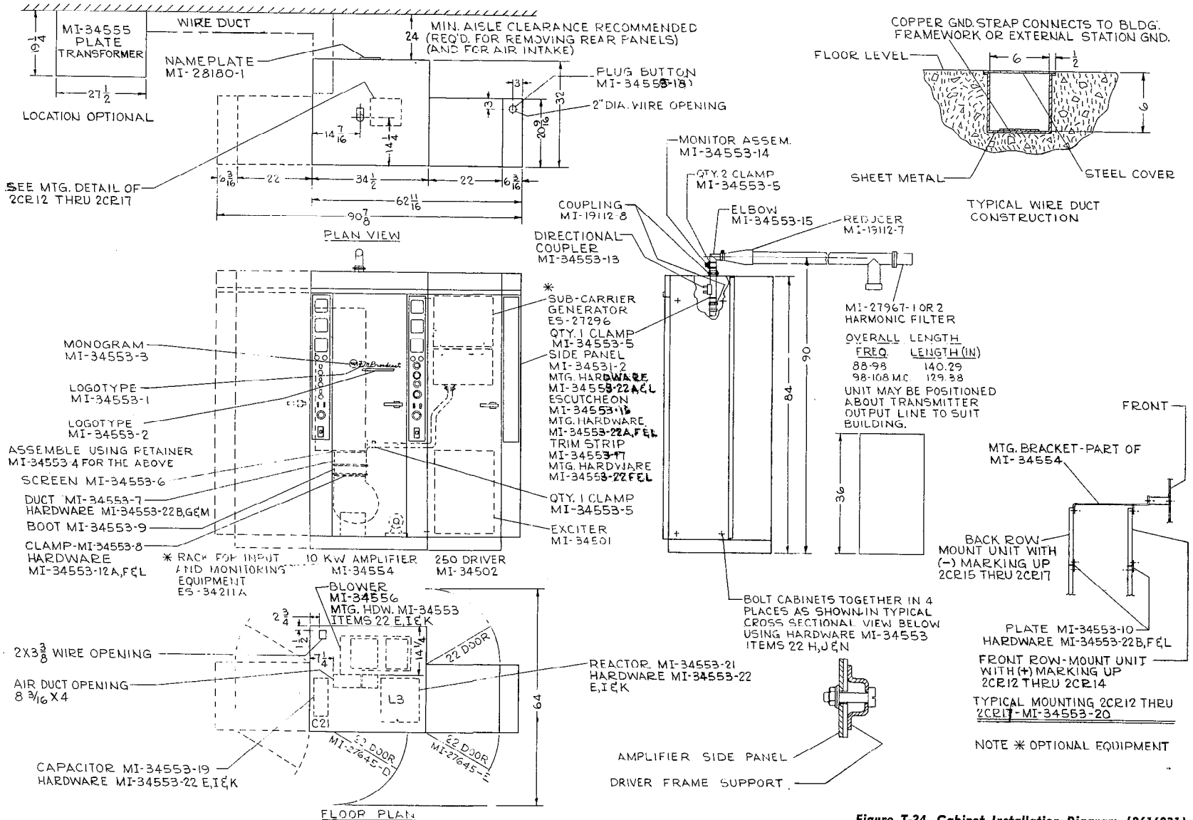
Figure T-24. Cabinet Installation Diagram (8616031)
