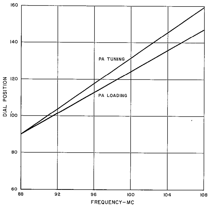
Figure T-7. PA Plate Tuning and Plate Loading Curve
