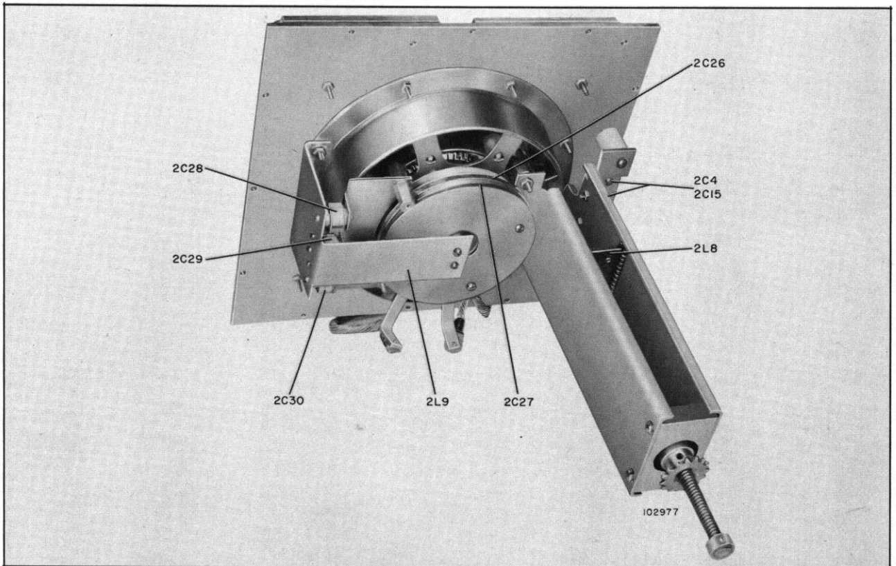
Figure T-19. PA Tube Socket, Bottom View
