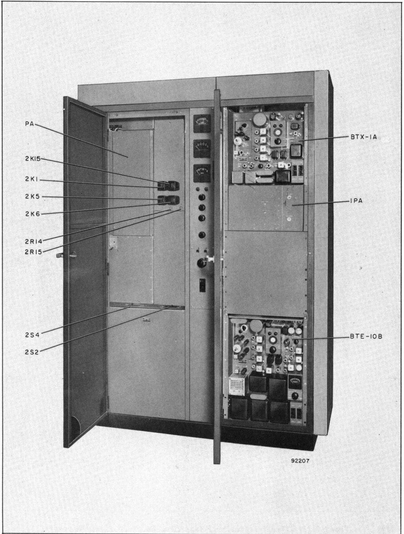
Figure T-12. BT-10D FM Transmitter, Front View, Doors Open
