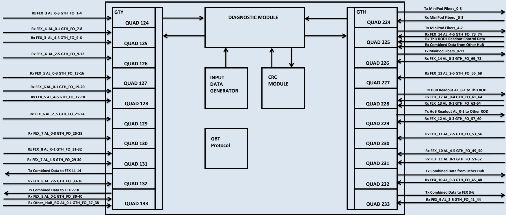
HUB FW DIAGRAM FPGA: xcvu125-flvc2104-1-i
