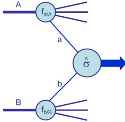
Figure 1. Diagrammatic structure of a generic hard scattering process.
