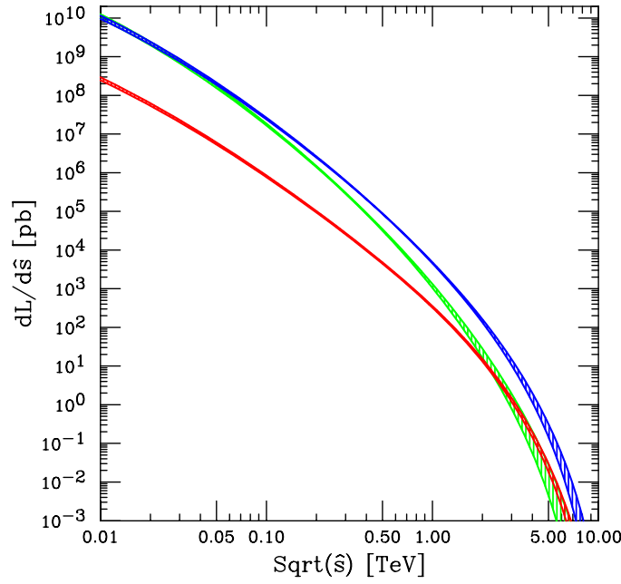
Figure 69. The parton-parton luminosity \left[\frac{dL_{ij}}{d\hat{s}}\right] in picobarns, integrated over y . Green= gg , Blue= \sum_i(gq_i + g\bar{q}_i + q_i g + \bar{q}_i g) , Red= \sum_i(q_i \bar{q}_i + \bar{q}_i q_i) , where the sum runs over the five quark flavours d, u, s, c, b .
