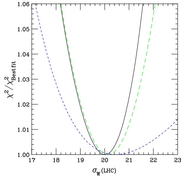
Figure 81. Predicted total cross section of W^+ + W^- production at the LHC for the fits obtained in the CTEQ stability study, compared to the MRST results. The overall pdf uncertainty of the prediction is \sim 5\% , as observed in Figure 77.
