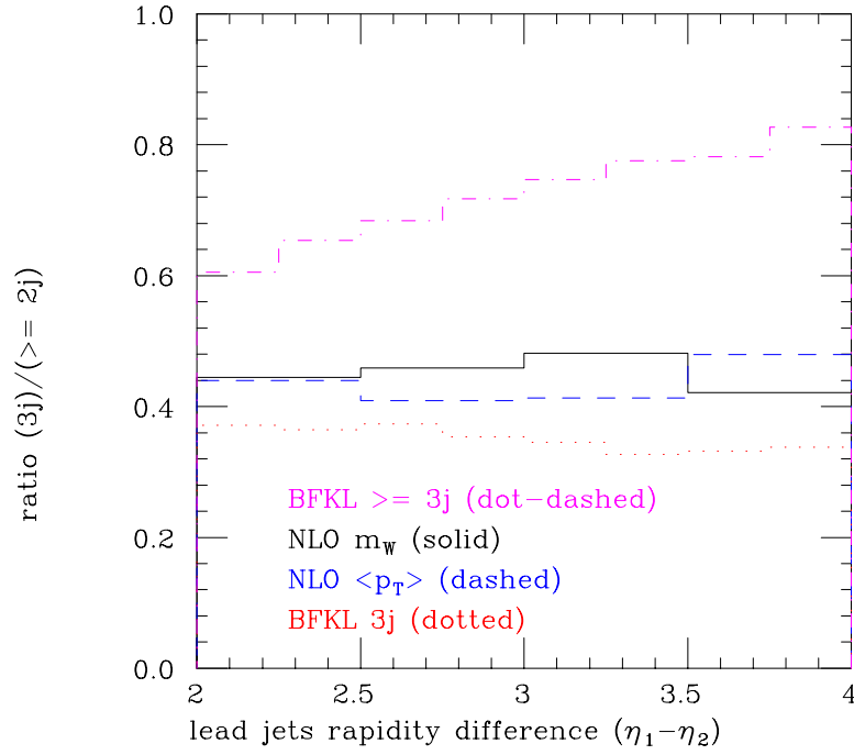
Figure 92. The rate for production of a third (or more) jet in W + \geq 2 jet events as a function of the rapidity separation of the two leading jets. A cut of 20 GeV has been placed on all jets. Predictions are shown from MCFM using two values for the renormalization and factorization scale, and using the BFKL formalism, requiring either that there be exactly 3 jets or 3 or more jets.
