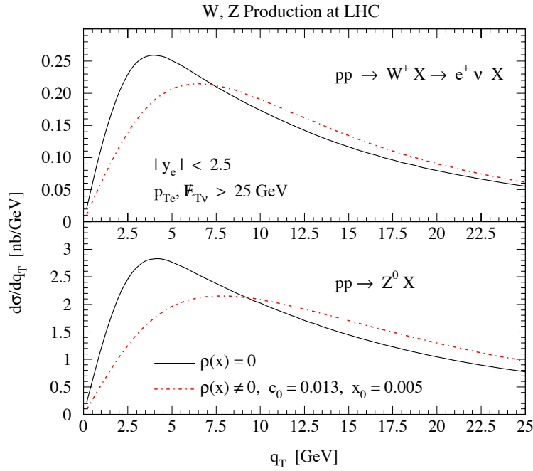
Figure 90. The predictions for the transverse momentum distributions for W and Z production with and without the p_T -broadening effects.
