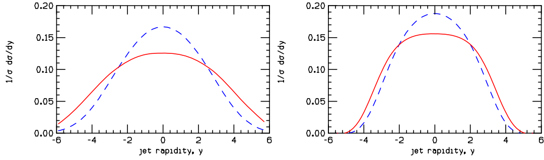
Figure 9. The rapidity distribution of the final state parton found in a lowest order calculation of the W + 1 jet cross section at the LHC. The parton is required to have a p_T larger than 2 GeV (left) or 50 GeV (right). Contributions from q\bar{q} annihilation (solid red line) and the qg process (dashed blue line) are shown separately.
