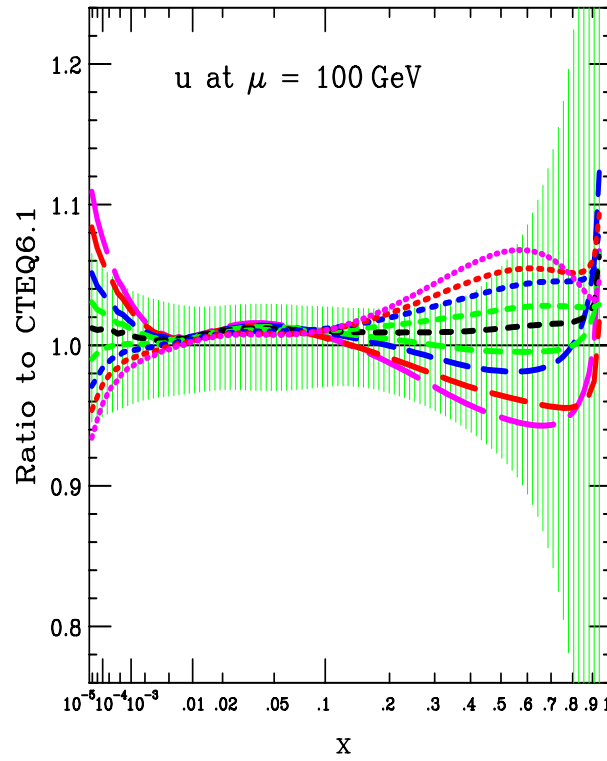
Figure 34. Variation of the up quark distribution for different values of \alpha_S . \alpha_S varies from 0.110 (short-dash) to 0.124 (long-dash) in increments of 0.002.
