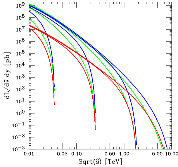
Figure 74. d(\text{Luminosity})/dy at rapidities (right to left) y = 0, 2, 4, 6 . Green= gg , Blue= \sum_i (qq_i + gq_i + q_i g + q_i q_i) , Red= \sum_i (q_i q_i + q_i q_i) , where the sum runs over the five quark flavours d, u, s, c, b .
