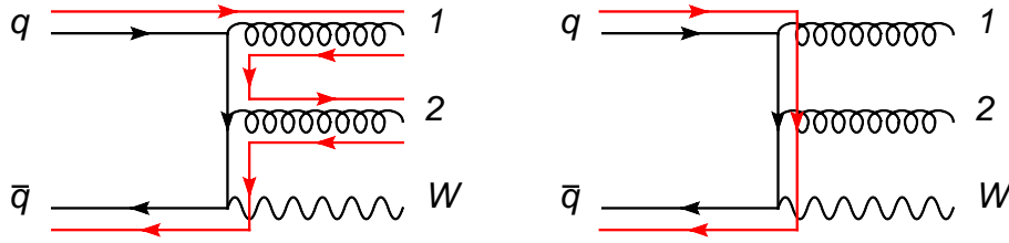
Figure 12. Two examples of colour flow in a W + 2 jet event, shown in red. In the left hand diagram, a leading colour flow is shown. The right-hand diagram depicts the sub-leading colour flow resulting from interference.
