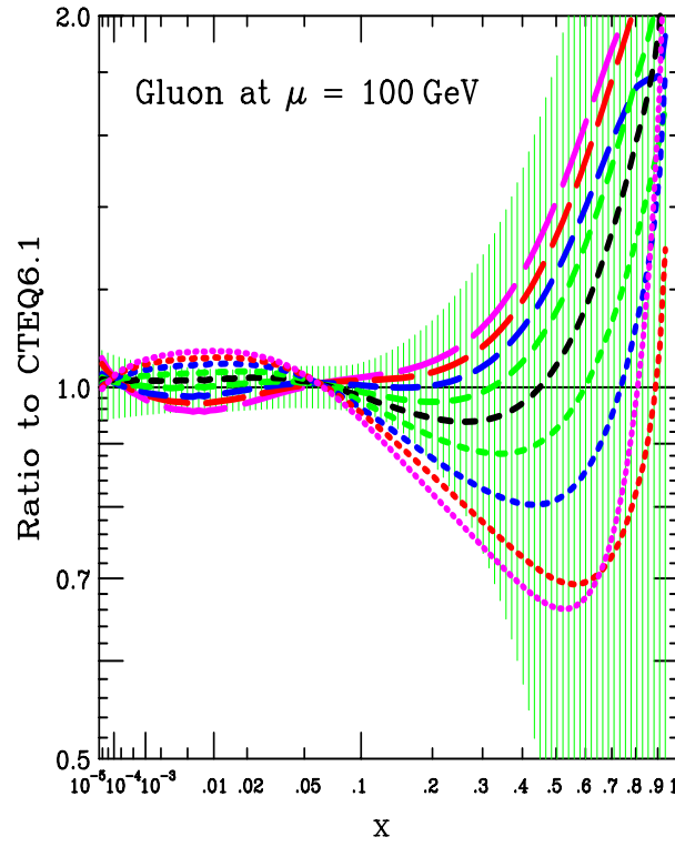
Figure 35. Variation of the gluon distribution for different values of \alpha_S . \alpha_S varies from 0.110 (short-dash) to 0.124 (long-dash) in increments of 0.002.
