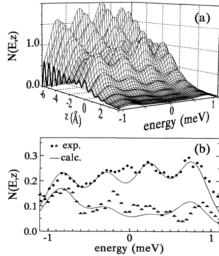
FIG. 4. Thermally broadened bound state contribution to the local density of states. (a) N(E,z) calculated from the dG-SJ model. (b) The experimental bound state contributions derived from Fig. 2, curves B (triangles) and E (dots). The experimental curves are compared to the curves z=-4.3 Å and z=-2.0 Å, respectively, from (a). The amplitude of the calculated curves has been reduced by a scaling factor of 0.25.
