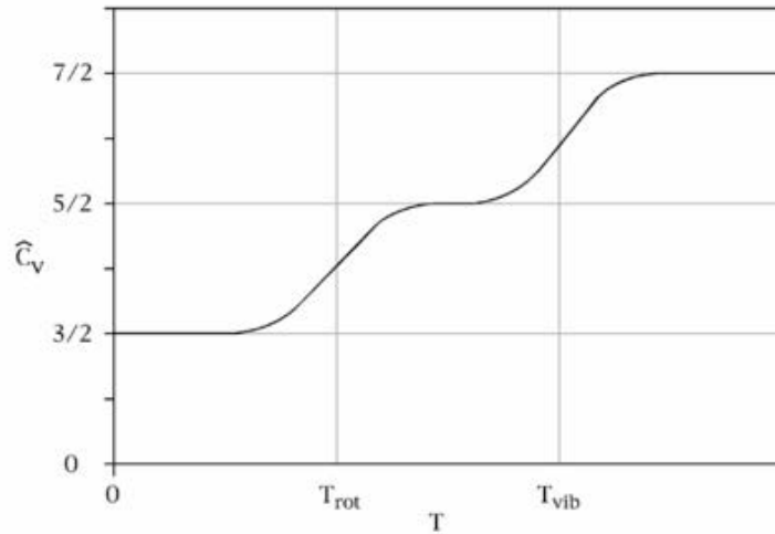
Figure 1: Constant-volume specific heat capacity of a diatomic gas (idealised), as a function of temperature.
