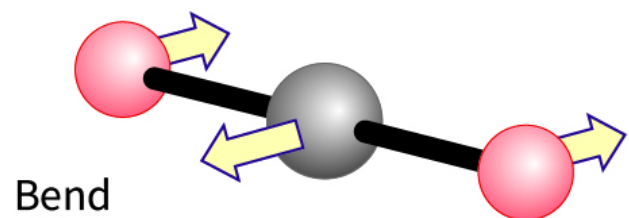
Figure 3: The four vibration modes of CO_2 .
