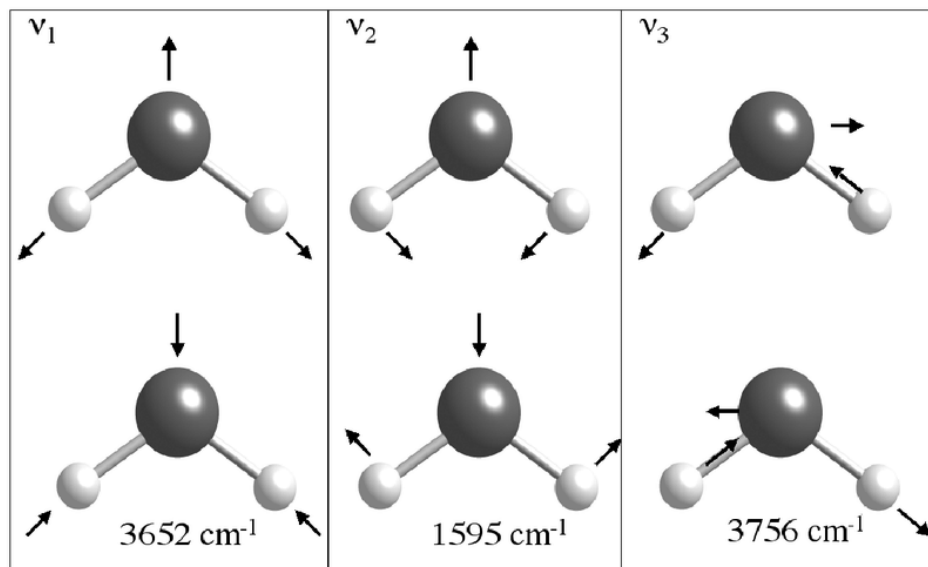
Figure 2: The three vibration modes of H_2O , with wave the corresponding wave numbers 1/\lambda .
