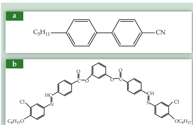
Figure 2. Chemical structures of organic molecules whose different shapes affect the character of the liquid crystal they form. (a) 5CB (pentyl cyanobiphenyl), a rod-shaped molecule. (b) A banana-shaped molecule.
