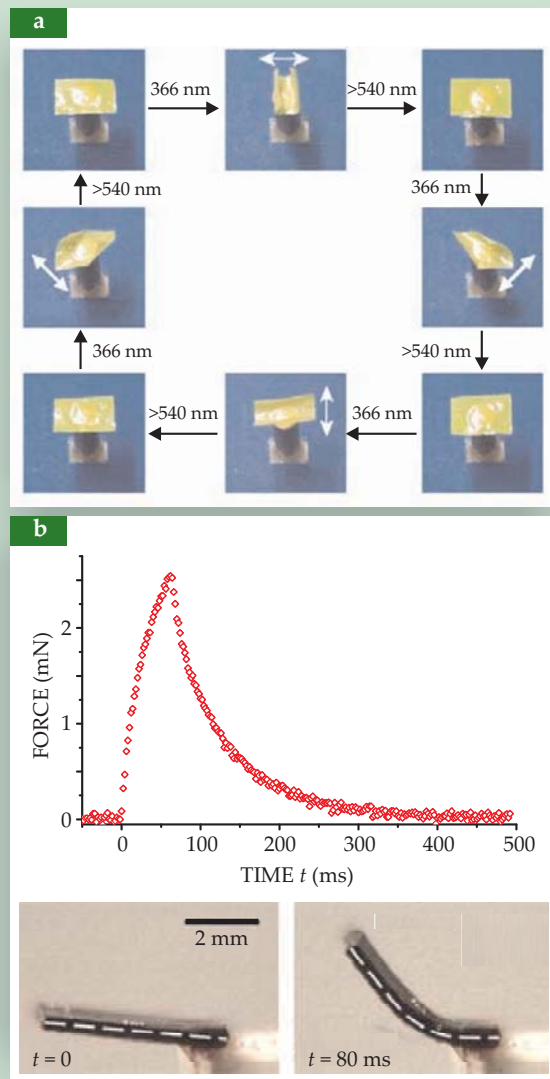
Figure 6. Light-induced deformation of liquid-crystal elastomers. (a) UV illumination at a wavelength of 366 nm makes a polydomain nematic network curl around the direction of polarization. The film then uncurls when illuminated by visible light. The film's reaction time is of order 10 seconds. (Courtesy of T. Ikeda.) (b) Photoactivation at 514 nm of a dye-doped monodomain nematic elastomer. 6 When illumination is stopped after 50 ms, the bending force decays with a relaxation time of about 75 ms.
